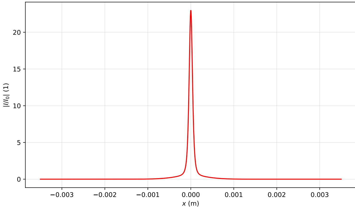
Intensity profile I(x, y = 0, z = 0.716)/I_0 , P_{in}=3.0P_{cr} , artificial time
